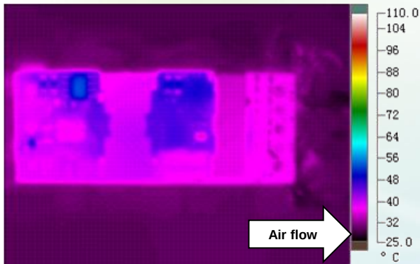
Figure 5: Thermal plot with airflow from V_{in} to V_{out} ( T_A = 25^\circ\text{C} ( 77^\circ\text{F} ); Airflow = 1 m/s (200 FLM); V_{in} = 48\text{ V} ; V_{out} = 5\text{ V} ; I_{out} = 10\text{ A} )
