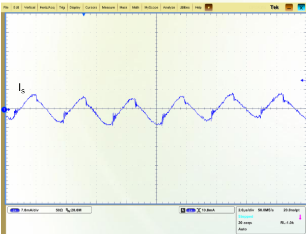
Figure 9: Input reflected ripple current (for point A in the test set-up diagram, V_{\text{in}} = 48\text{ V} , V_{\text{out}} = 5\text{ V} , I_{\text{out}} = 10\text{ A} )
