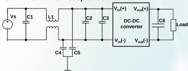
Figure 22: EMC test set-up diagram
