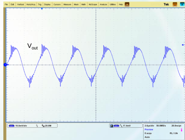
Figure 10: Output voltage ripple (for point B in the test set-up diagram, V_{\text{in}} = 48\text{ V} , V_{\text{out}} = 5\text{ V} , I_{\text{out}} = 10\text{ A} )
