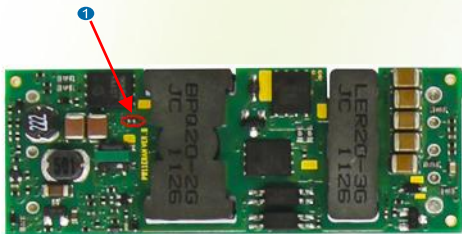
Figure 23: Thermal test point
