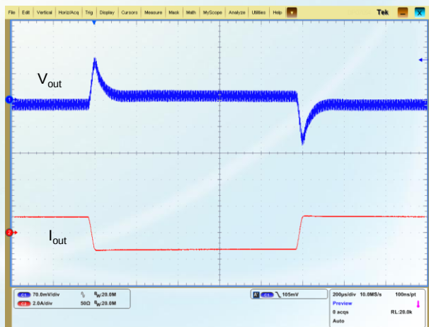
Figure 16: Output voltage dynamic response (Load: 50% - 75% - 50%, di/dt = 0.1\text{ A}/\mu\text{s} )
