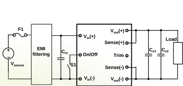
Figure 8: Typical circuit applications
