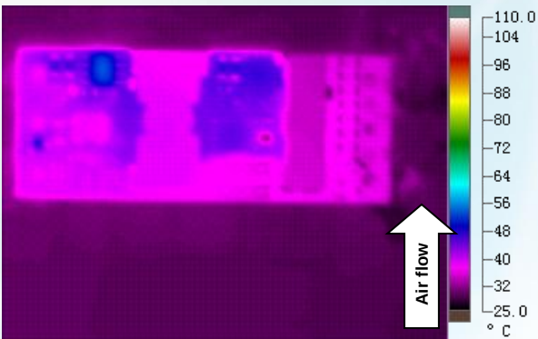
Figure 6: Thermal plot with airflow from V_{in}(-) to V_{in}(+) ( T_A = 25^\circ\text{C} ( 77^\circ\text{F} ); Airflow = 1 m/s (200 FLM); V_{in} = 48\text{ V} ; V_{out} = 5\text{ V} ; I_{out} = 10\text{ A} )
