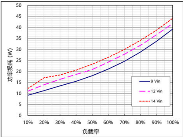
功率损耗 ( T_A=25^{\circ}C , V_{out}=1.0V , I_{out}=300A )
