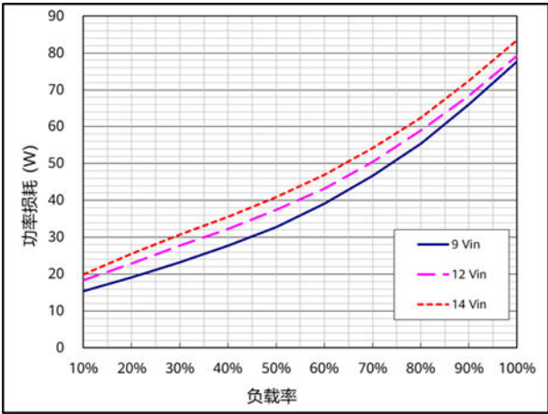
功率损耗 ( T_A=25^{\circ}\text{C} , V_{\text{out}}=1.0\text{V} , I_{\text{out}}=500\text{A} )
