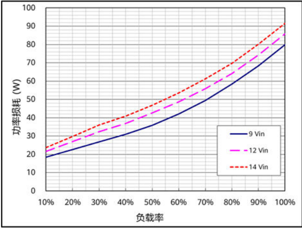
功率损耗 ( T_A=25^{\circ}\text{C} , V_{\text{out}}=1.0\text{V} , I_{\text{out}}=600\text{A} )
