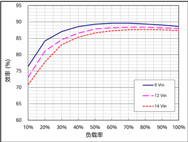
效率 ( T_A=25^{\circ}C , V_{out}=1.0V , I_{out}=300A )
