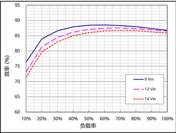
效率 ( T_A=25^{\circ}\text{C} , V_{\text{out}}=1.0\text{V} , I_{\text{out}}=500\text{A} )
