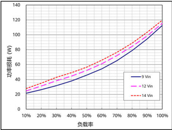
功率损耗 ( T_A=25^{\circ}\text{C} , V_{\text{out}}=1.0\text{V} , I_{\text{out}}=700\text{A} )
