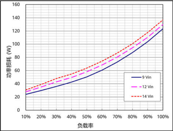
功率损耗 ( T_A=25^{\circ}\text{C} , V_{\text{out}}=1.0\text{V} , I_{\text{out}}=800\text{A} )
