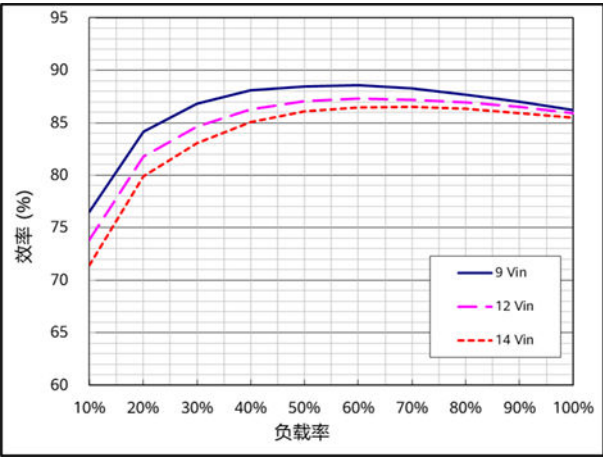
效率 ( T_A=25^{\circ}\text{C} , V_{\text{out}}=1.0\text{V} , I_{\text{out}}=700\text{A} )
