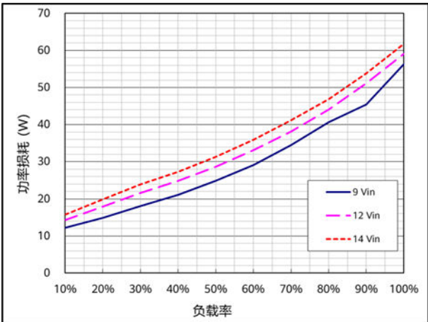
功率损耗 ( T_A=25^{\circ}C , V_{out}=1.0V , I_{out}=400A )
